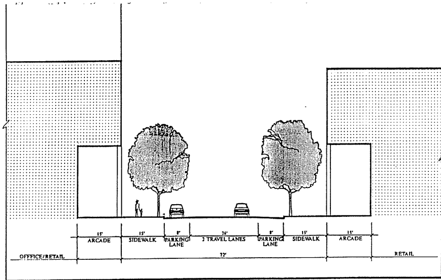
Montgomery Avenue Section
