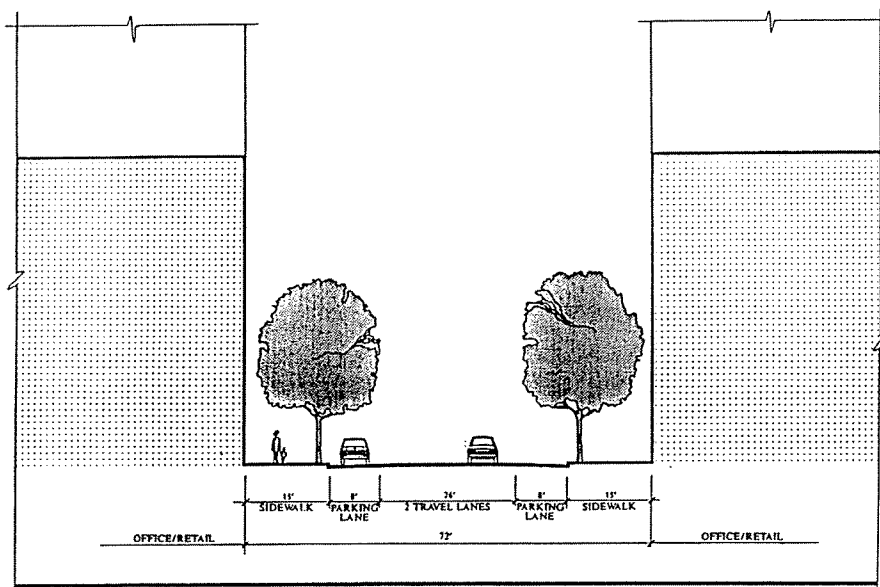
"Center" Street Section
