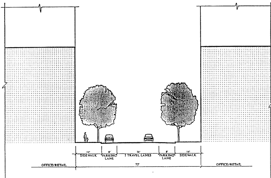
Maryland Avenue and Monroe Street Section
